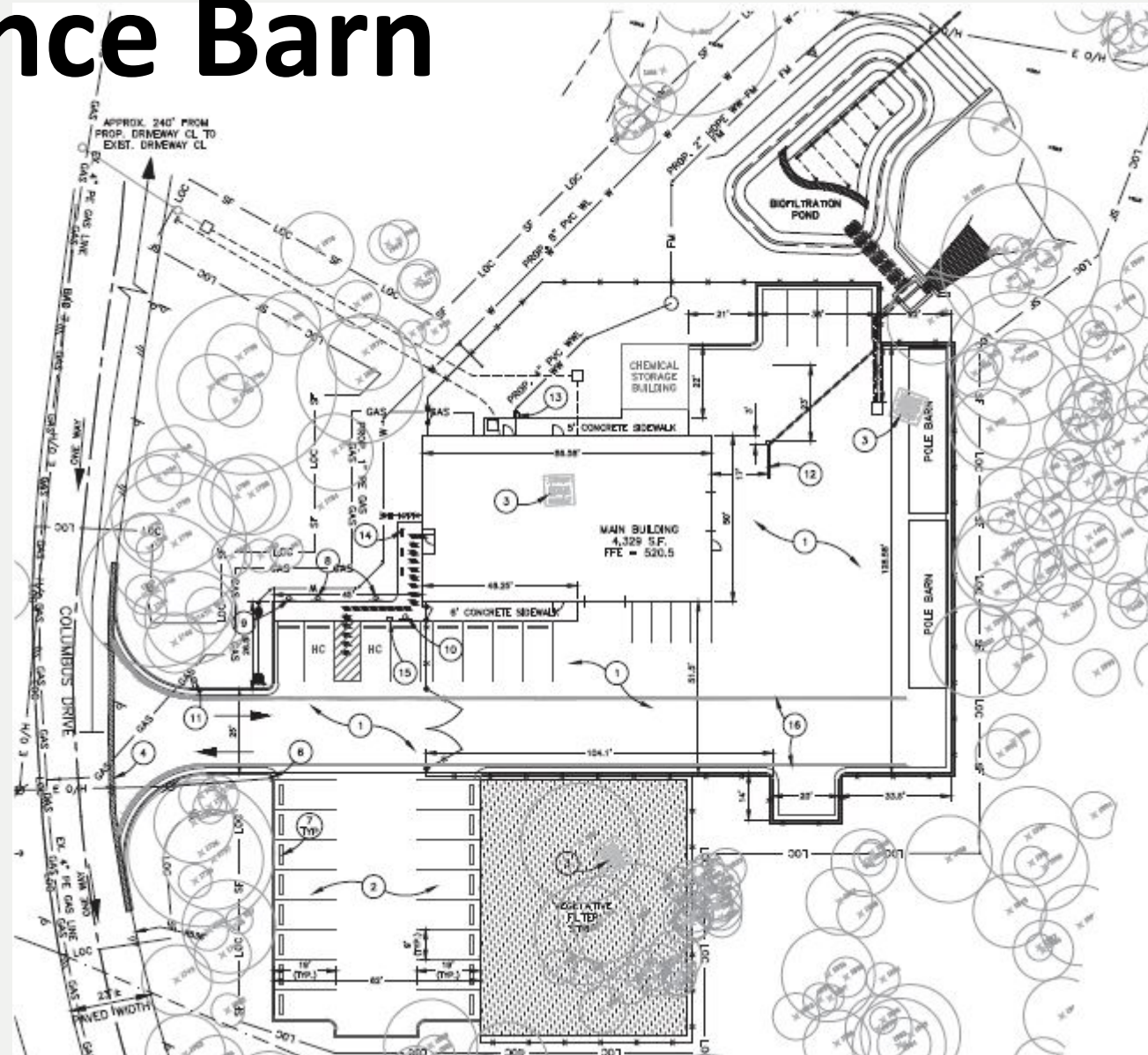
Maintenance Barn Site Plan
